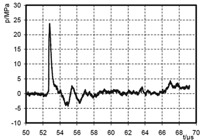
Figure 1. Pressure waveform for the Dermagold® unit at low energy. The plot shows the maximum and minimum pressures (p) created in megapascals (MPa) over time (t) in microseconds ( \mu s).
